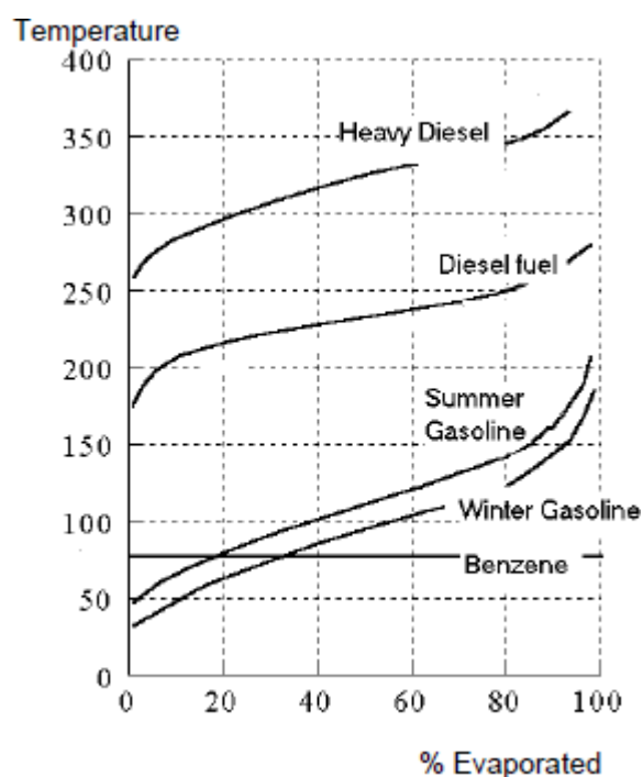
Fig. 12. Distillation curve
