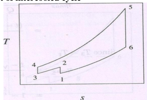
T-S diagram
