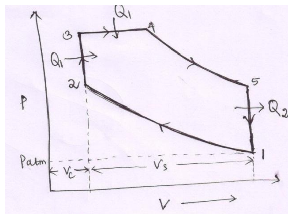
Fig. 9. Dual cycle
