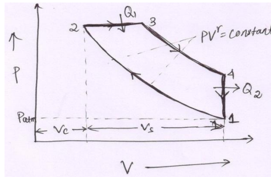
Fig. 8. Diesel cycle
