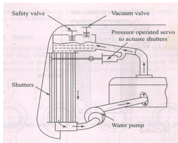
Fig. 39. Pressurised system
